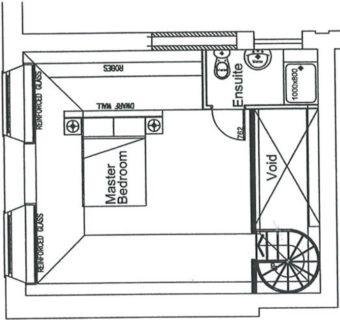
Apartment NO-4 LAYOUT FLOOR PLAN
